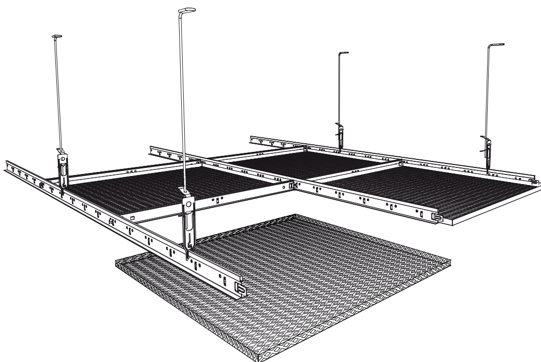
24 LINEAR REGULAR - T24 ribassato/lowered 15mm
