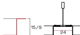
24 LINEAR REGULAR - T24 ribassato/lowered 15mm
