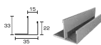
PROFILO | PROFILE 15 "F" L=3000mm
