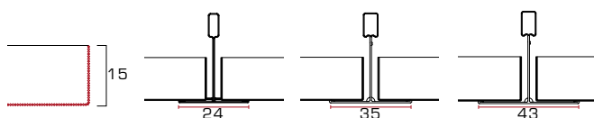
PLAN - T24 | T35 | T43
