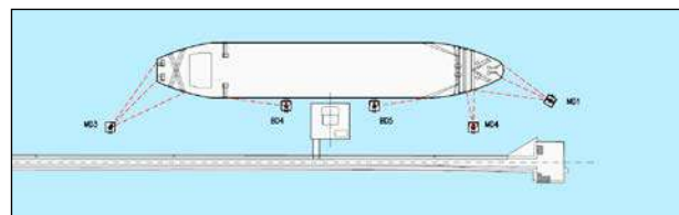
New Exxon berth - Plan view
