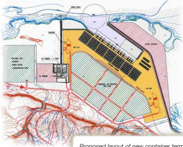
Proposed layout of new container terminal
