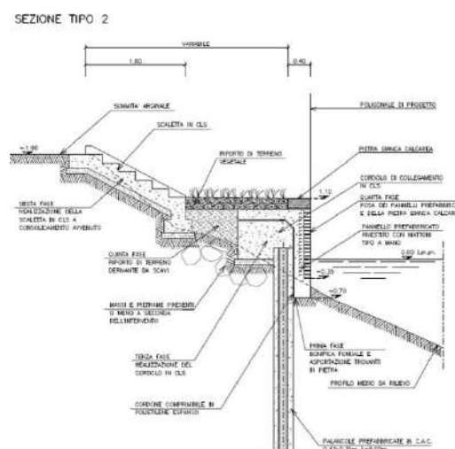
Concrete sheet-piling cross section
