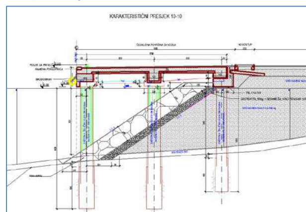
Fig.4. – Characteristic cross section of the maritime structure – conceptual design
