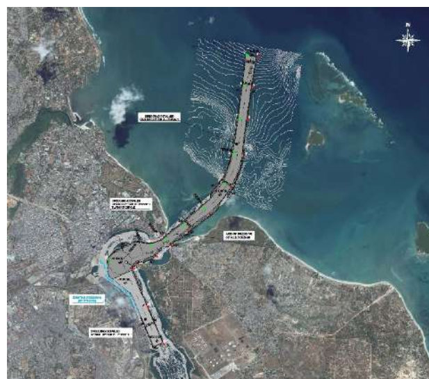
Detailed design of dredging of the port of Dar es Salaam: Option B – Phase 1 – General layout
