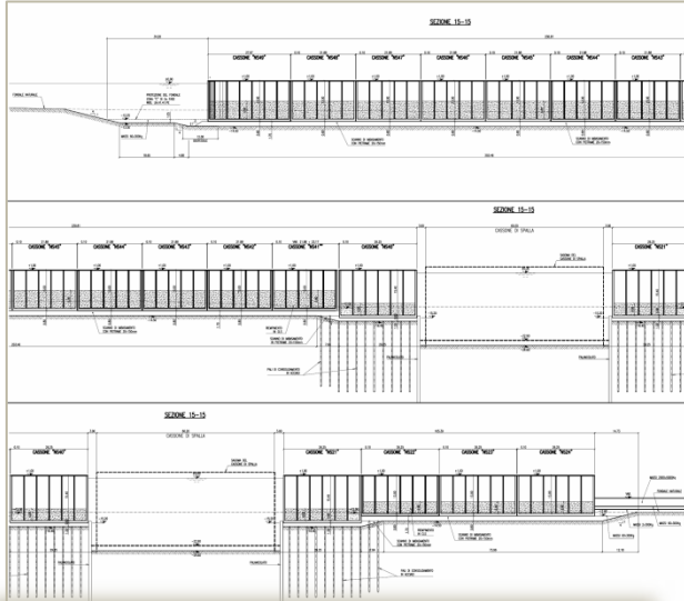
Cross-section of the South abutment caissons at Lido San Nicolò inlet.
