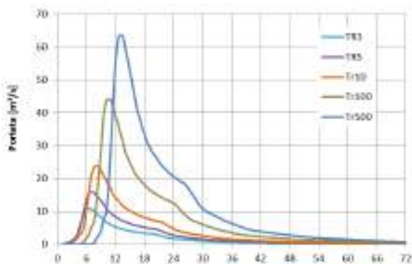
Design hydrograph for different Return period
