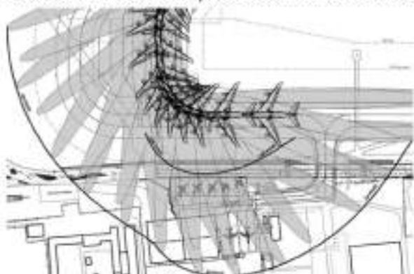
Detection of area to be protected from aircraft Jet
