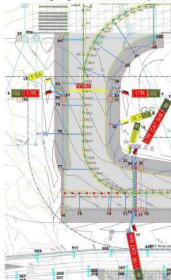
Details of aircraft General Aviation apron
