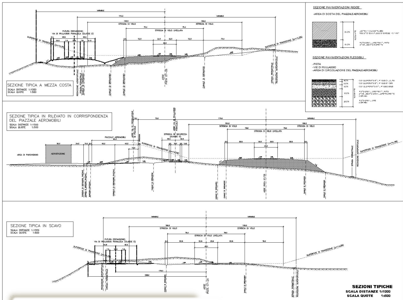
Typical sections of runway, taxiways and aircraft
