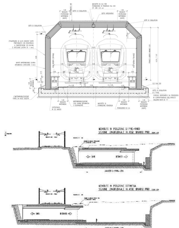
cutting the relevant embankment with no interference to the track and the rail service, as in the following figure
