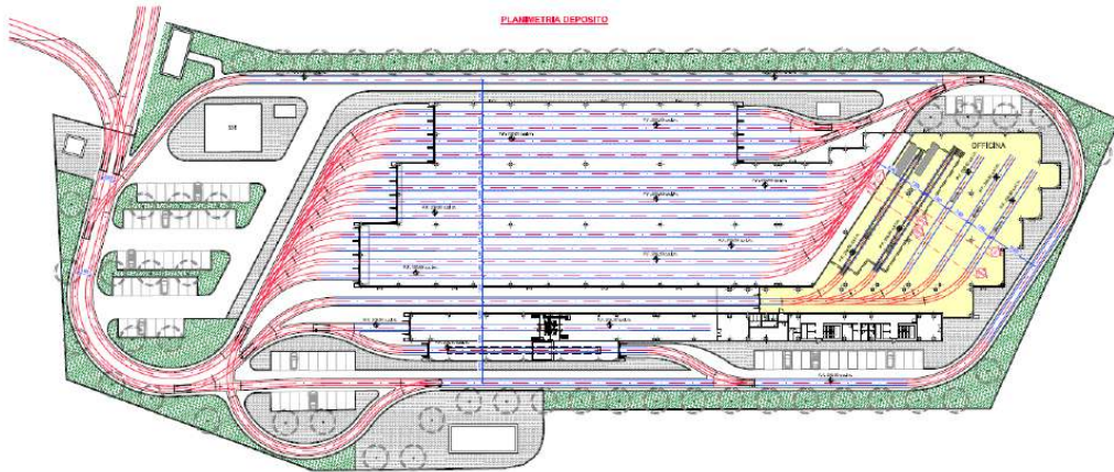
Layout of the depot/workshop
